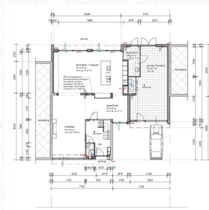
Fig 2. Begane grond
